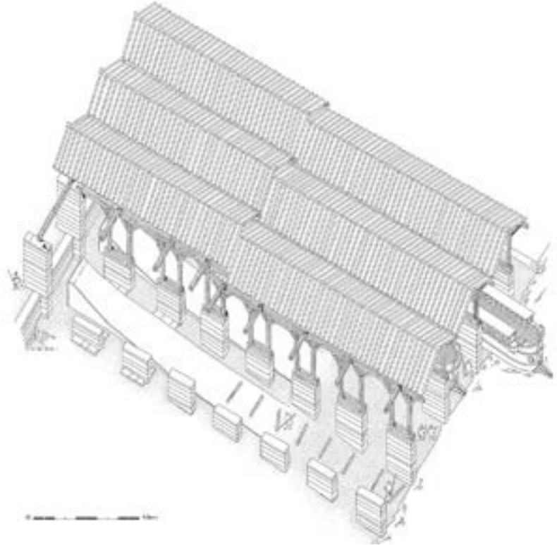
Reconstruction of the shipsheds of the military port, Kition-Bamboula, 4 th century BC. © O. Callot, Archives of the Archaeological Mission of Kition and Salamis.
